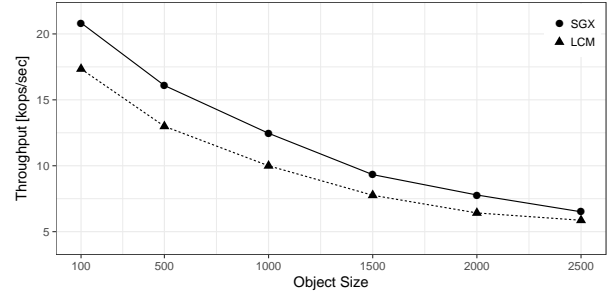
Fig. 4. Throughput with different object sizes with async disk writes.
