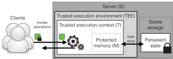
Fig. 1. System model comprising trusted clients, a potentially misbehaving server S that hosts a trusted execution context T .
