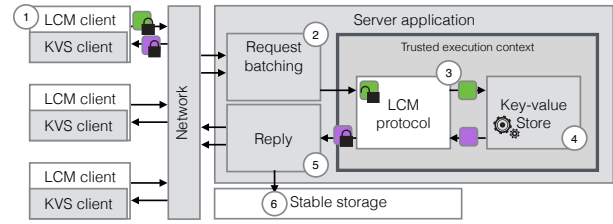
Fig. 3. The prototype architecture of an enclave based key-value store protected with LCM.
