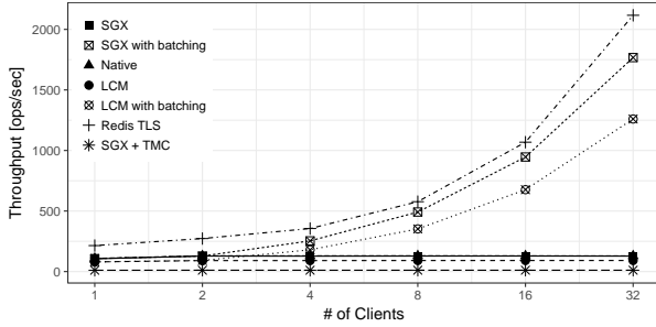
Fig. 6. Throughput with different numbers of clients with sync disk writes.
