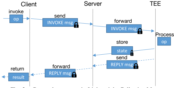
Fig. 2. Protocol messages in Lightweight Collective Memory
