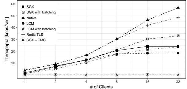
Fig. 5. Throughput with different numbers of clients with async disk writes.
